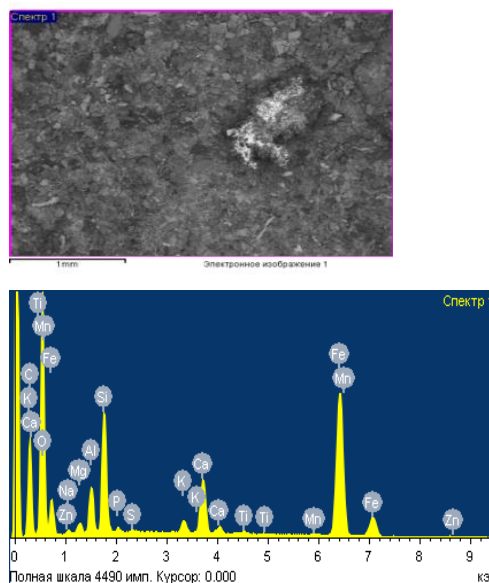
Figure 2 - The quantitative composition of the components elements in corrosion-scale incrustation taken from the surface of the plastic pipe of Aris and their structure
